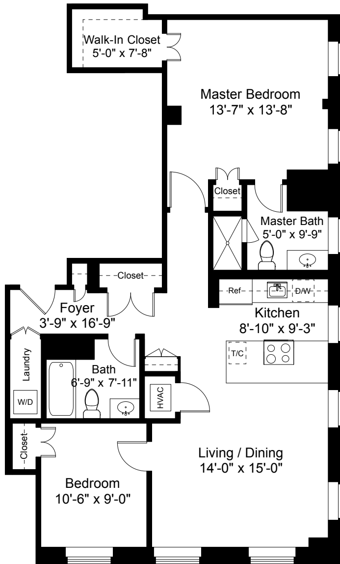
Unit 7A Floor Plan Ceiling Height = 8'-7"
