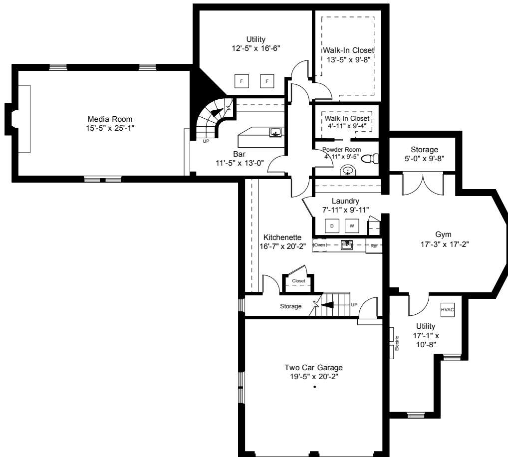
Lower Level Plan Ceiling Height = 7'-4"
