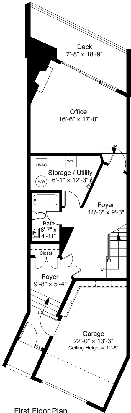
First Floor Plan Ceiling Height = 8'-0"
