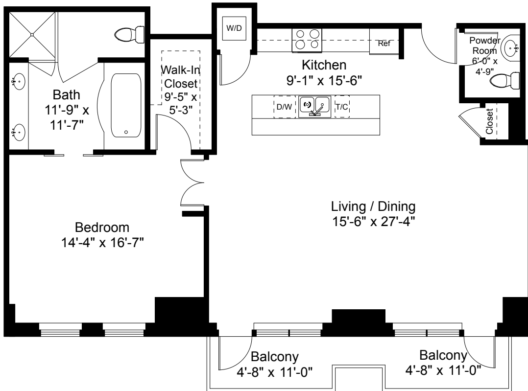
Unit 4507 Floor Plan Ceiling Height = 8'-0"
