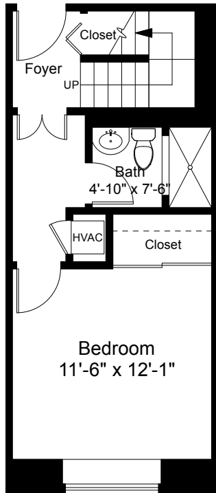
First Floor Plan Ceiling Height = 7'-9"
