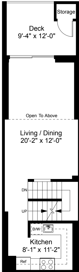
Second Floor Plan Ceiling Height = 7'-5"
