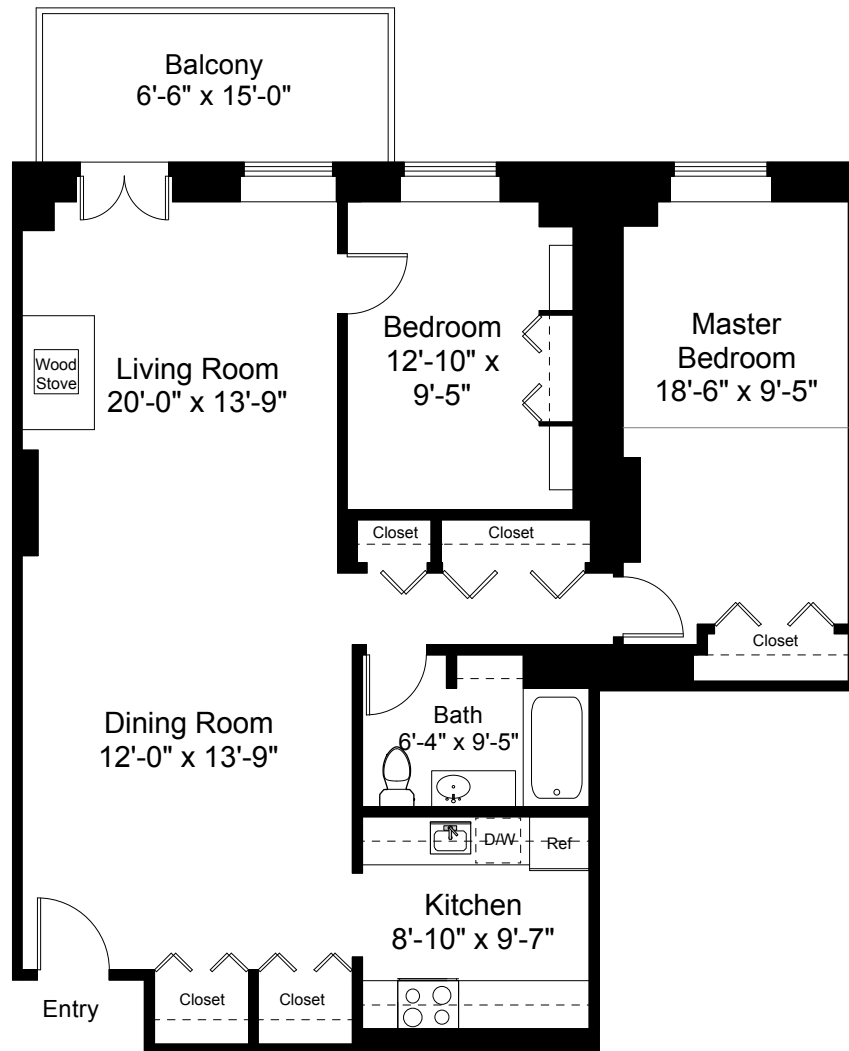
Unit 424 Floor Plan Ceiling Height = 9'-6"
