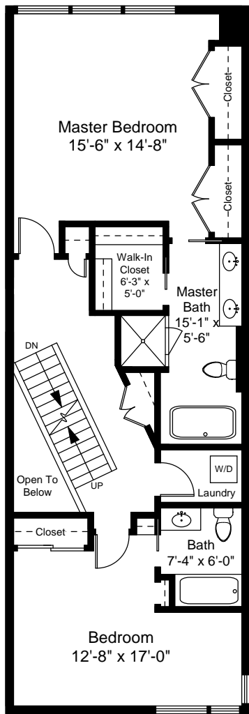
Third Floor Plan Ceiling Height = 7'-11"
