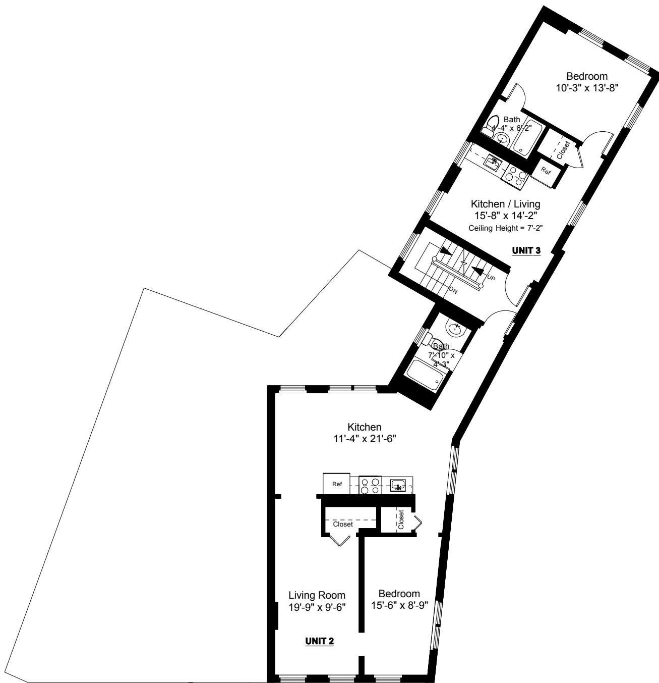
Second Floor Plan Ceiling Height = 7'-11"
