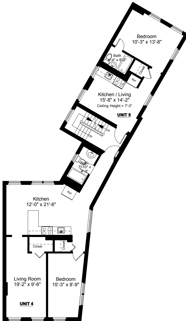
Third Floor Plan Ceiling Height = 8'-2"
