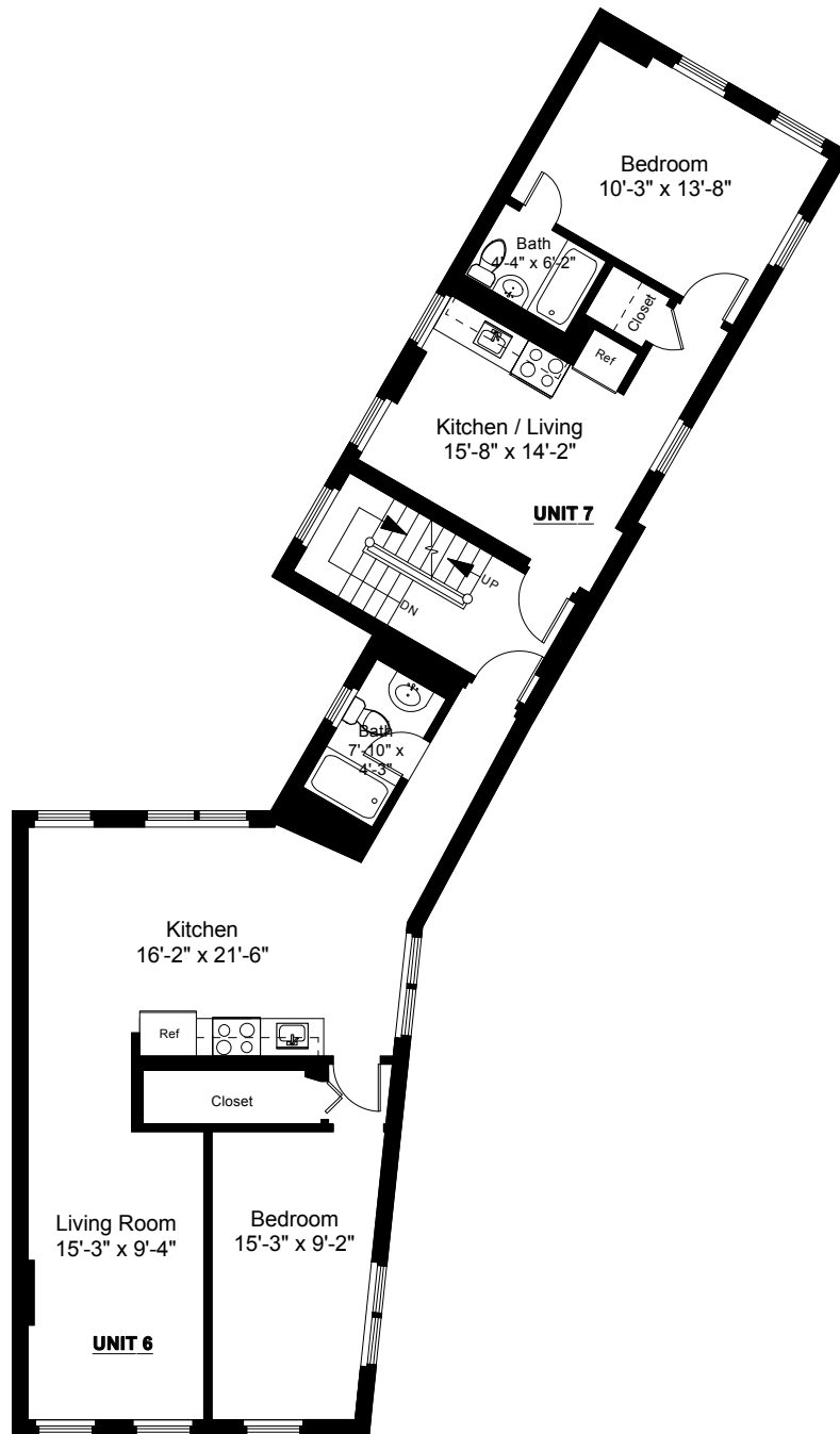
Fourth Floor Plan Ceiling Height = 7'-4"
