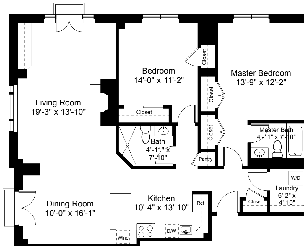
Unit 802 Floor Plan Ceiling Height = 8'-0"
