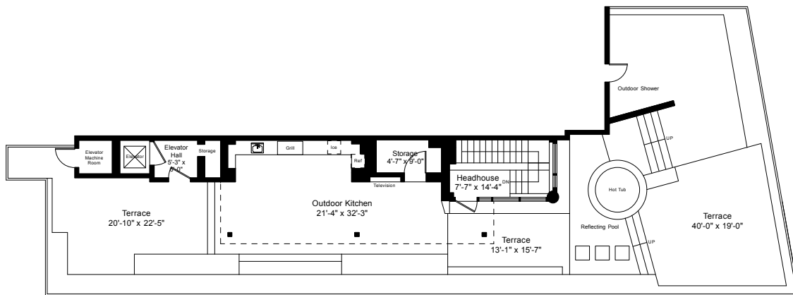
Rooftop Plan
