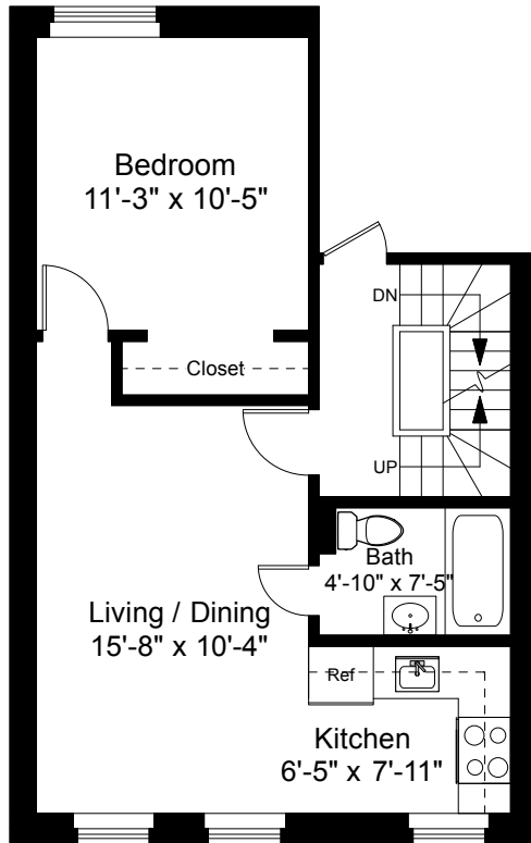
Unit 5 Floor Plan Ceiling Height = 9'-1"
