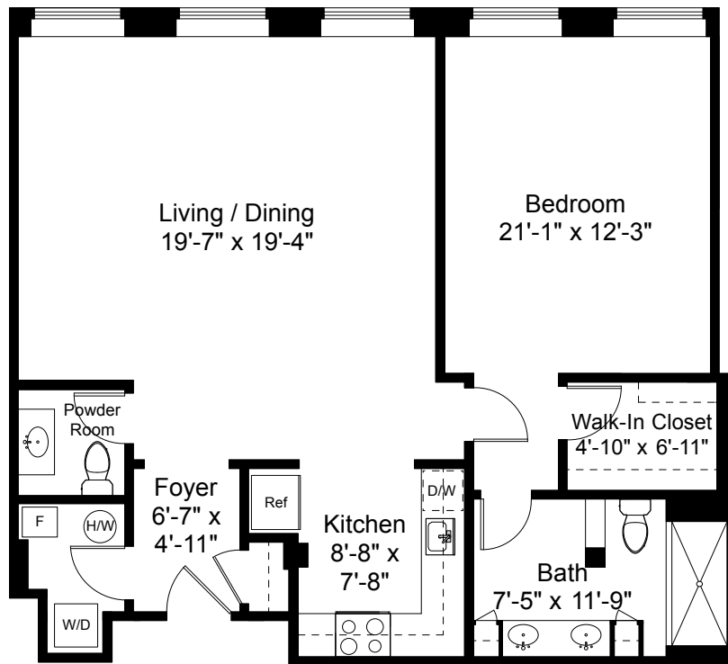
Unit 1B Floor Plan Ceiling Height = 12'-9"
