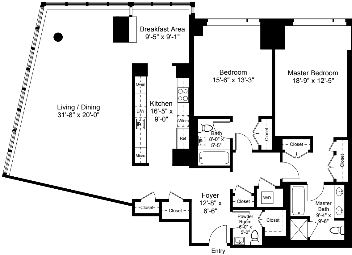
Unit 7D Floor Plan Ceiling Height = 9'-0"
