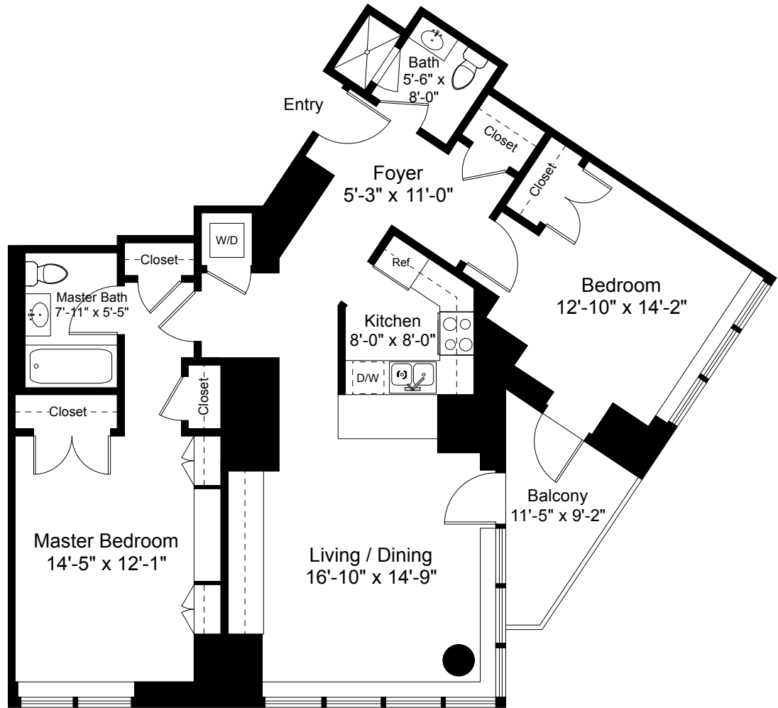
Unit 10D Floor Plan Ceiling Height = 8'-9"
