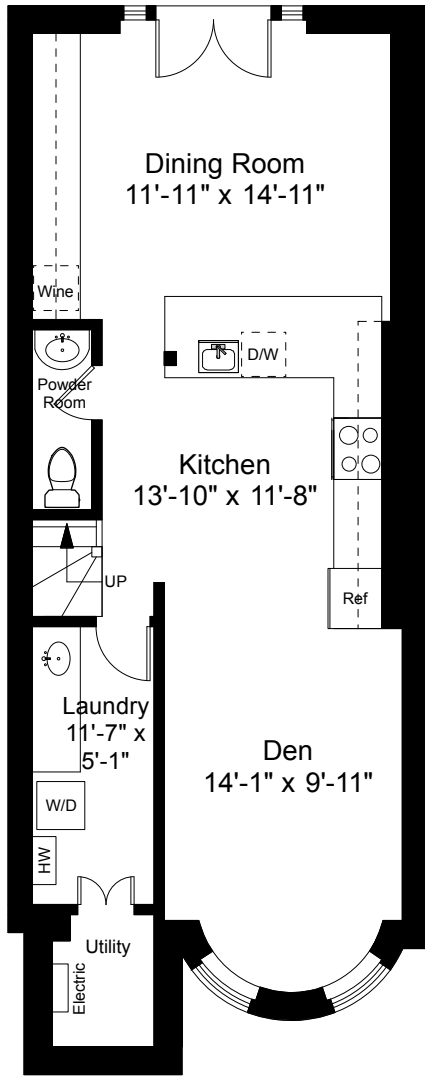
Garden Level Plan Ceiling Height = 8'-4"
