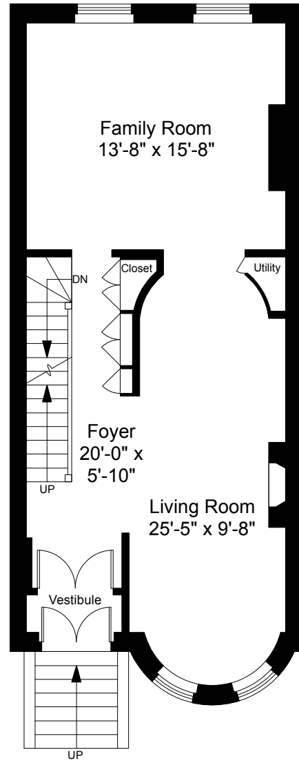
First Floor Plan Ceiling Height = 9'-10"
