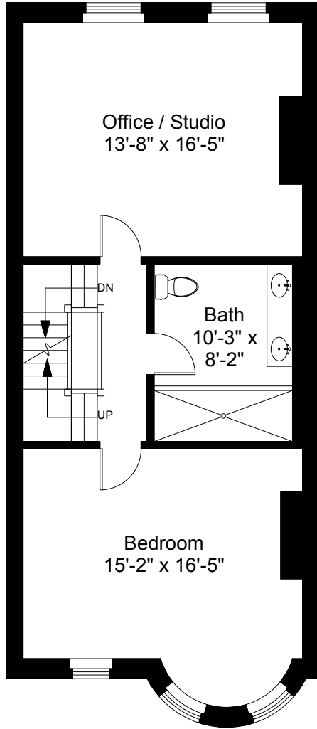
Second Floor Plan Ceiling Height = 8'-9"
